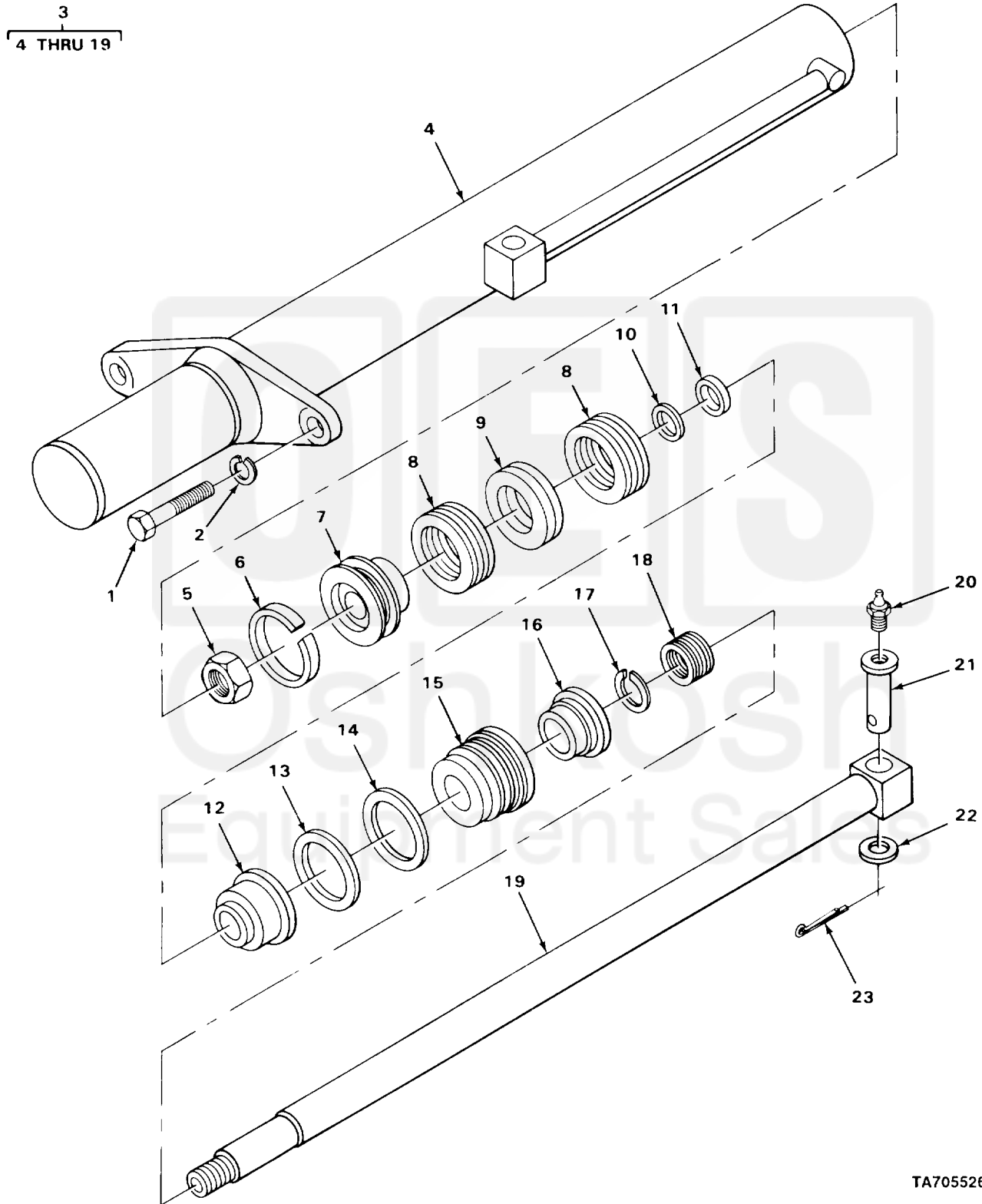
FIGURE 200 EXTENSION CYLINDER (MHE-200 AND MHE-222).
